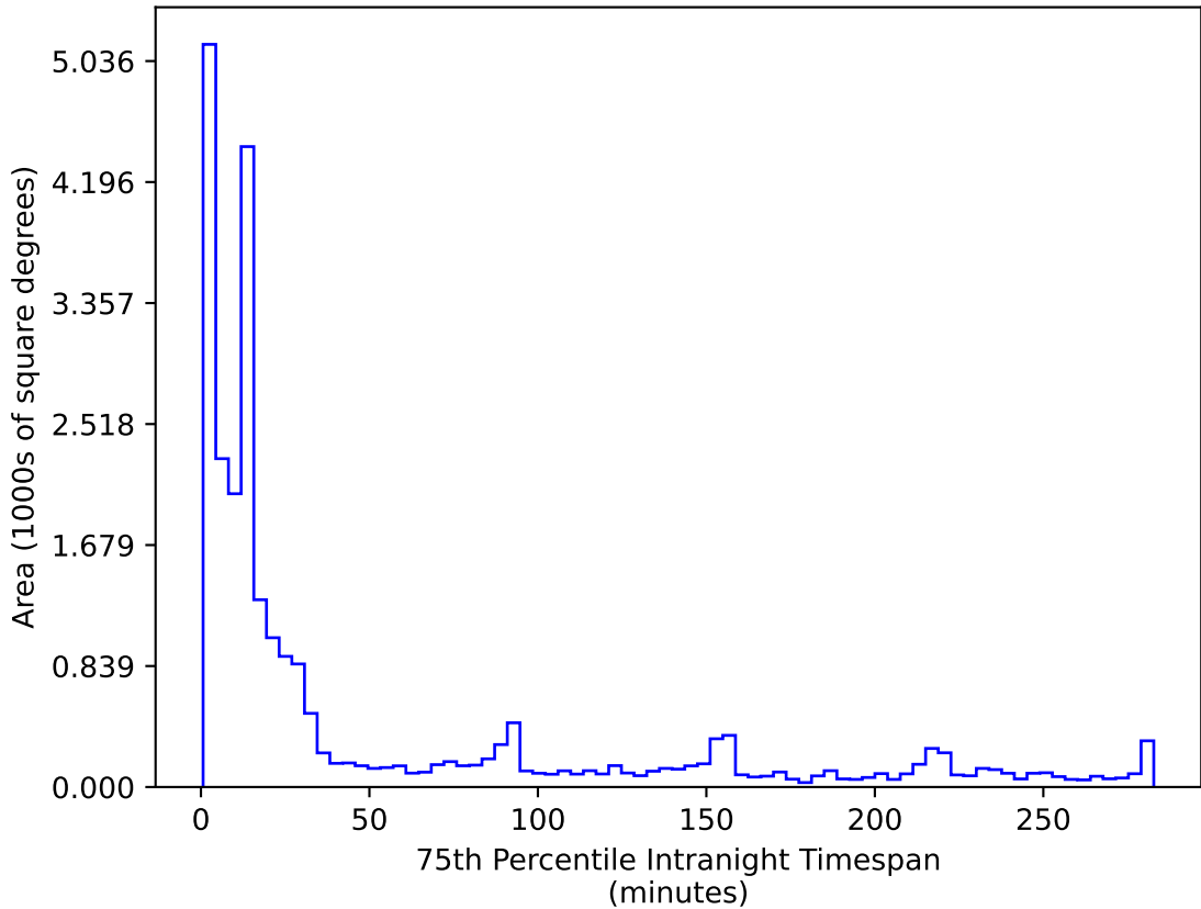
weather_cloudso10v3.4_10yrs All sky r band: 75th Percentile Intranight Timespan
