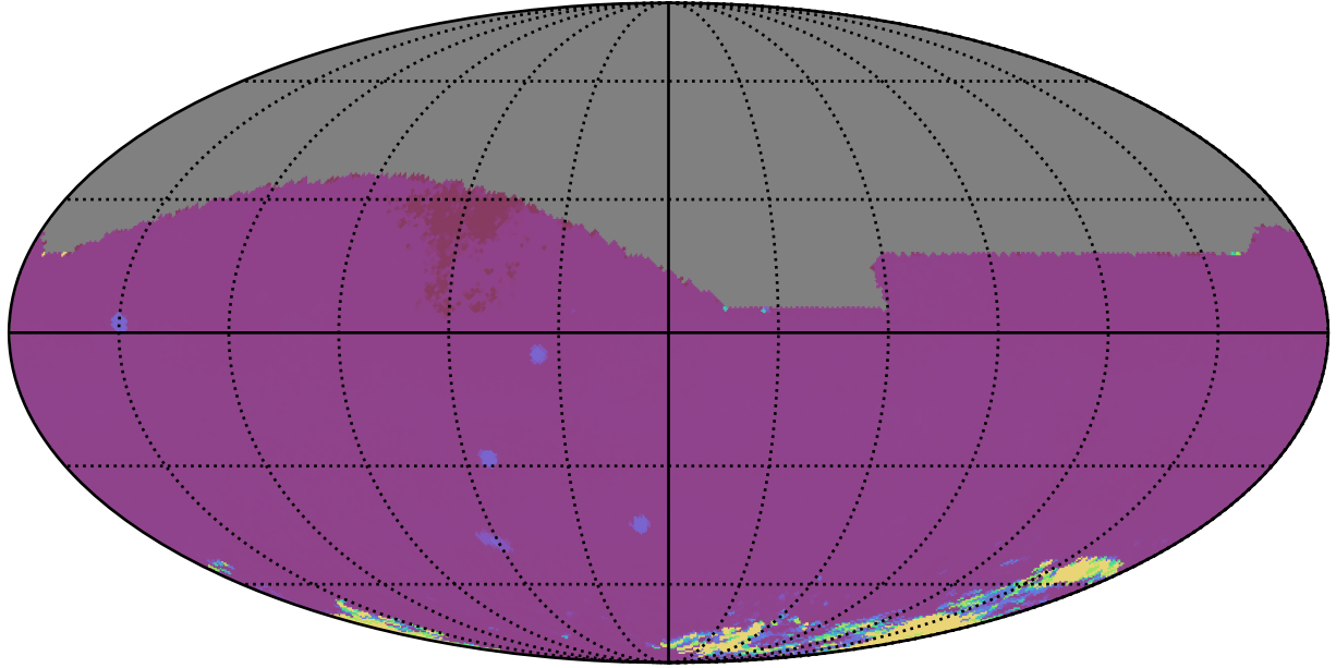
weather_cloudso10v3.4_10yrs All sky iz bands: 75th Percentile Intranight Timespan
