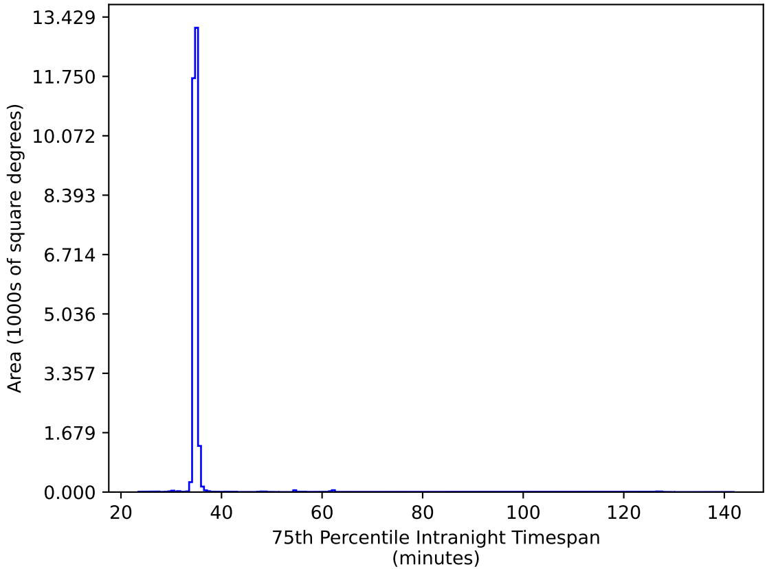
weather_cloudso10v3.4_10yrs All sky iz bands: 75th Percentile Intranight Timespan
