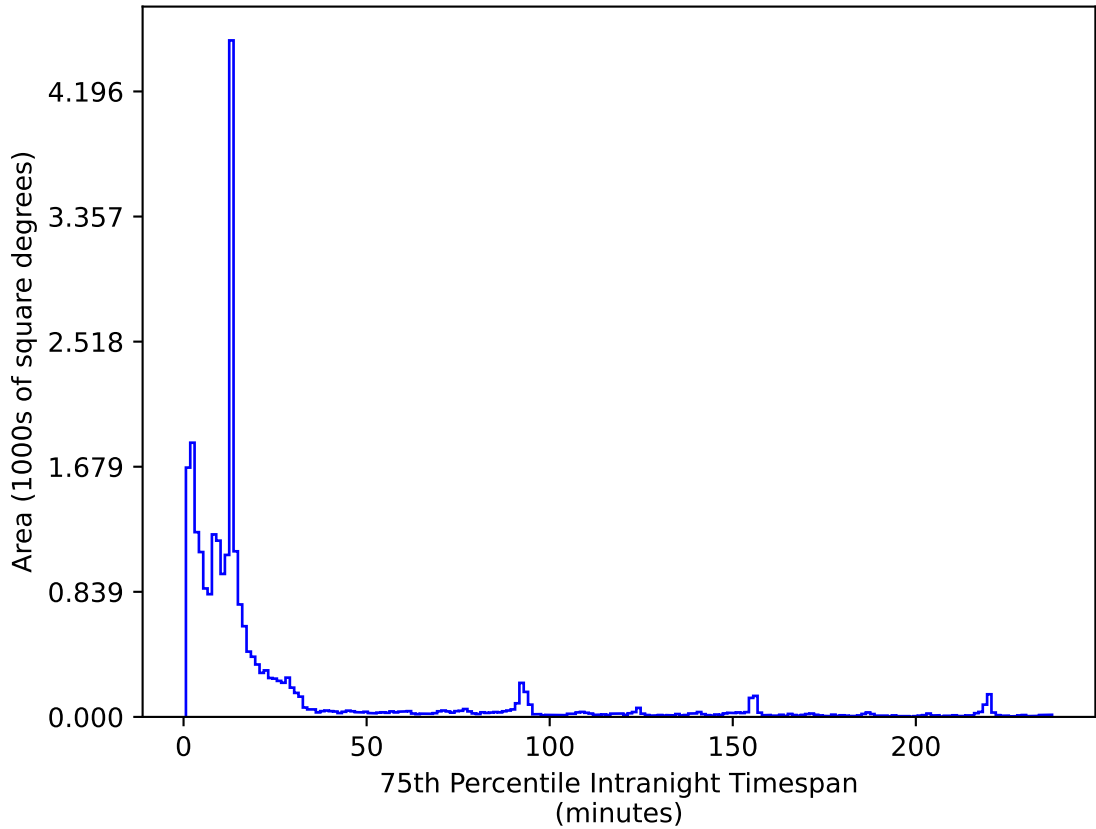
weather_cloudso10v3.4_10yrs All sky i band: 75th Percentile Intranight Timespan
