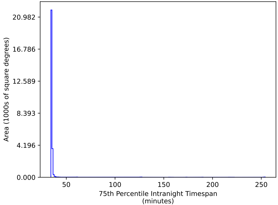
weather_cloudso10v3.4_10yrs All sky gr bands: 75th Percentile Intranight Timespan
