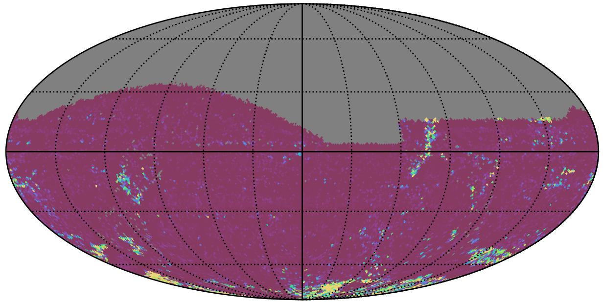
weather_cloudso10v3.4_10yrs All sky g band: 75th Percentile Intranight Timespan
