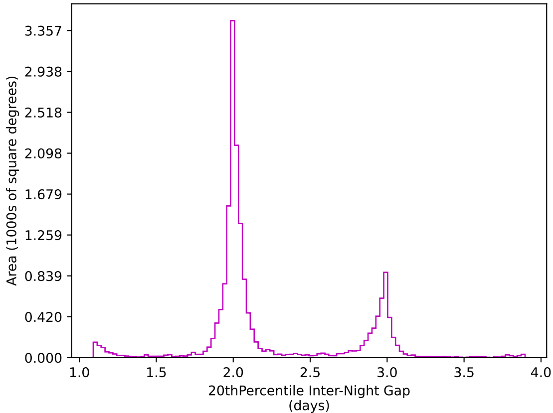
weather_cloudso10v3.4_10yrs WFD z band: 20thPercentile Inter-Night Gap
