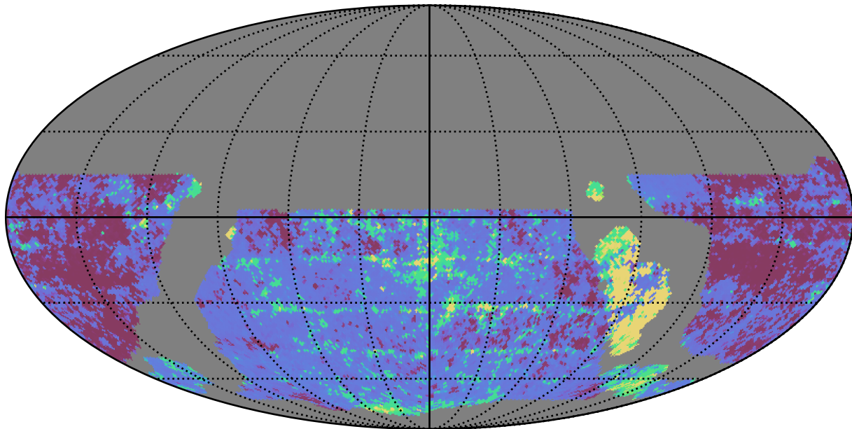
weather_cloudso10v3.4_10yrs WFD y band: 20thPercentile Inter-Night Gap
