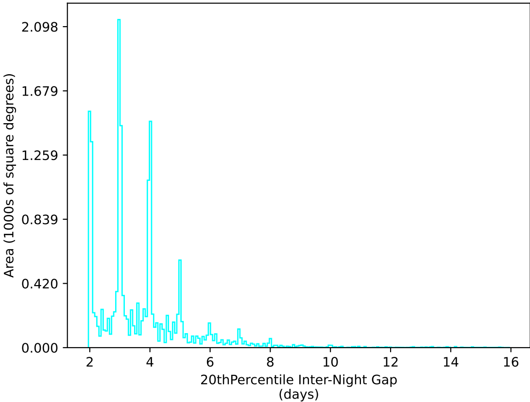
weather_cloudso10v3.4_10yrs WFD u band: 20thPercentile Inter-Night Gap
