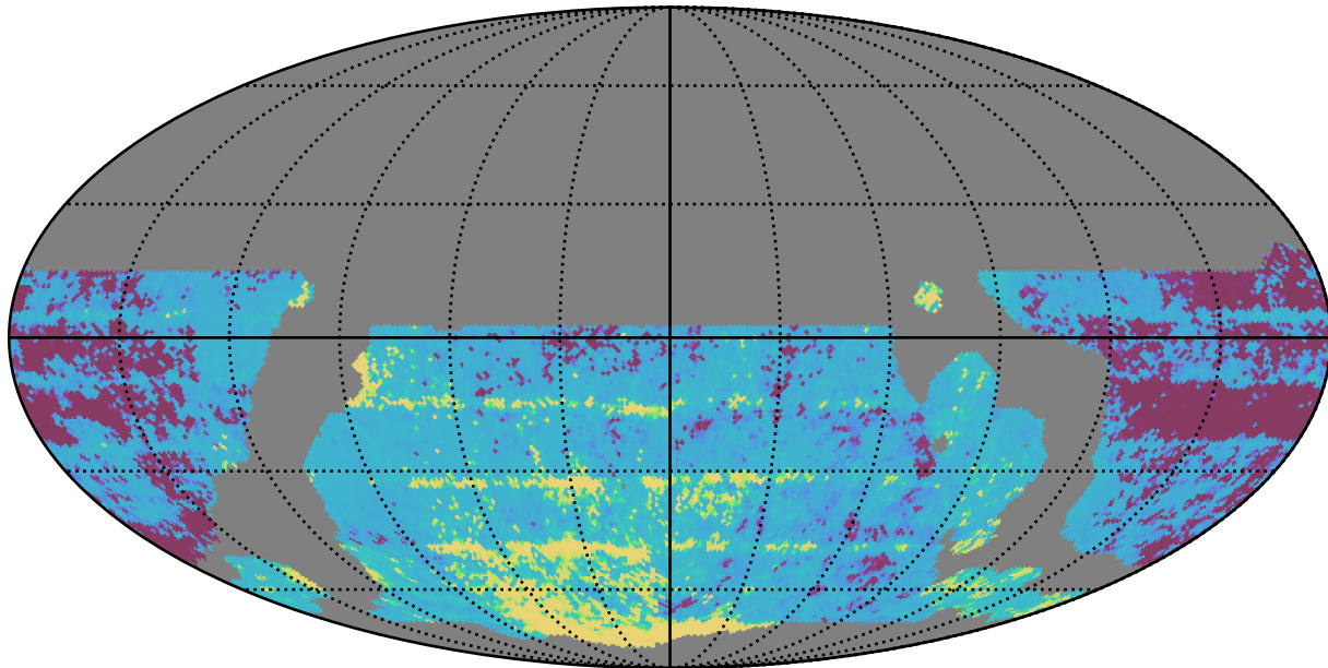
weather_cloudso10v3.4_10yrs WFD r band: 20thPercentile Inter-Night Gap
