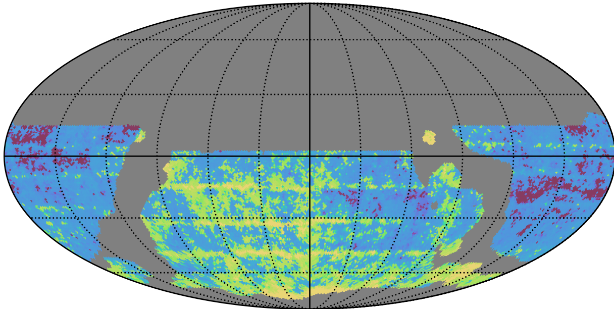
weather_cloudso10v3.4_10yrs WFD i band: 20thPercentile Inter-Night Gap
