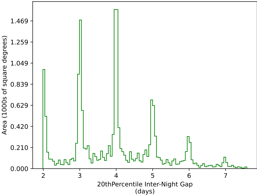
weather_cloudso10v3.4_10yrs WFD g band: 20thPercentile Inter-Night Gap
