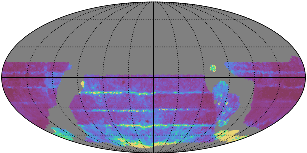
weather_cloudso10v3.4_10yrs WFD all bands: 20thPercentile Inter-Night Gap
