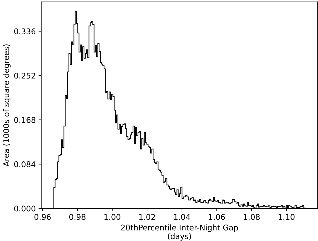
weather_cloudso10v3.4_10yrs WFD all bands: 20thPercentile Inter-Night Gap
