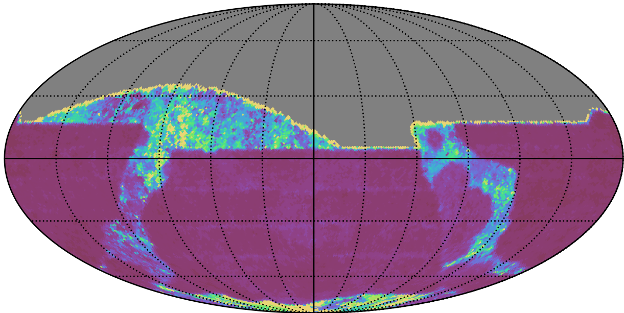
weather_cloudso10v3.4_10yrs All sky z band: 20thPercentile Inter-Night Gap
