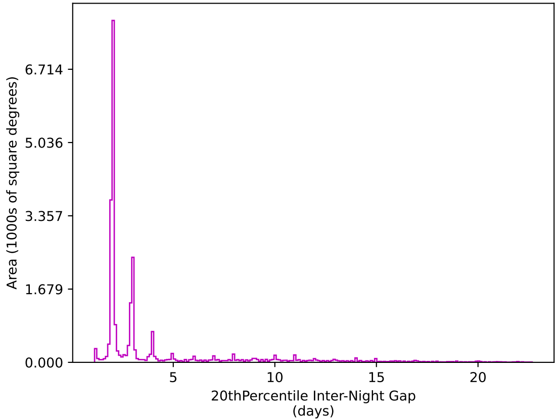
weather_cloudso10v3.4_10yrs All sky z band: 20thPercentile Inter-Night Gap
