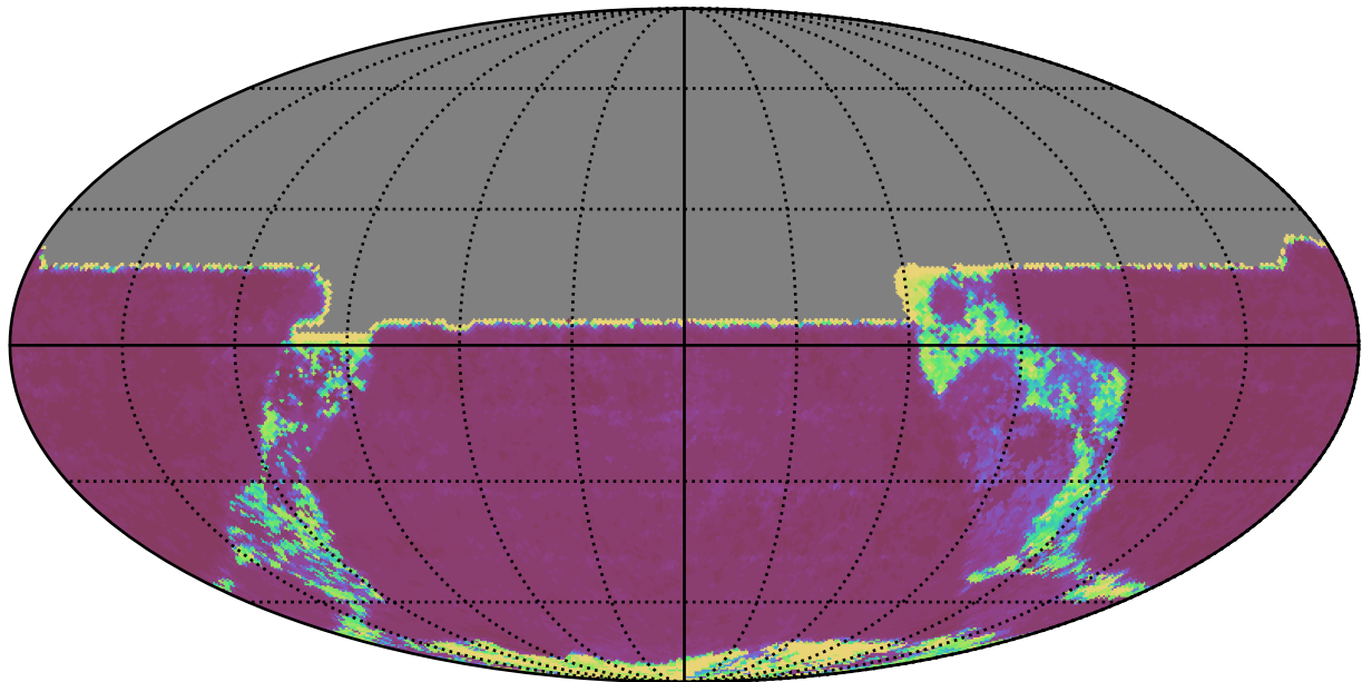
weather_cloudso10v3.4_10yrs All sky y band: 20thPercentile Inter-Night Gap
