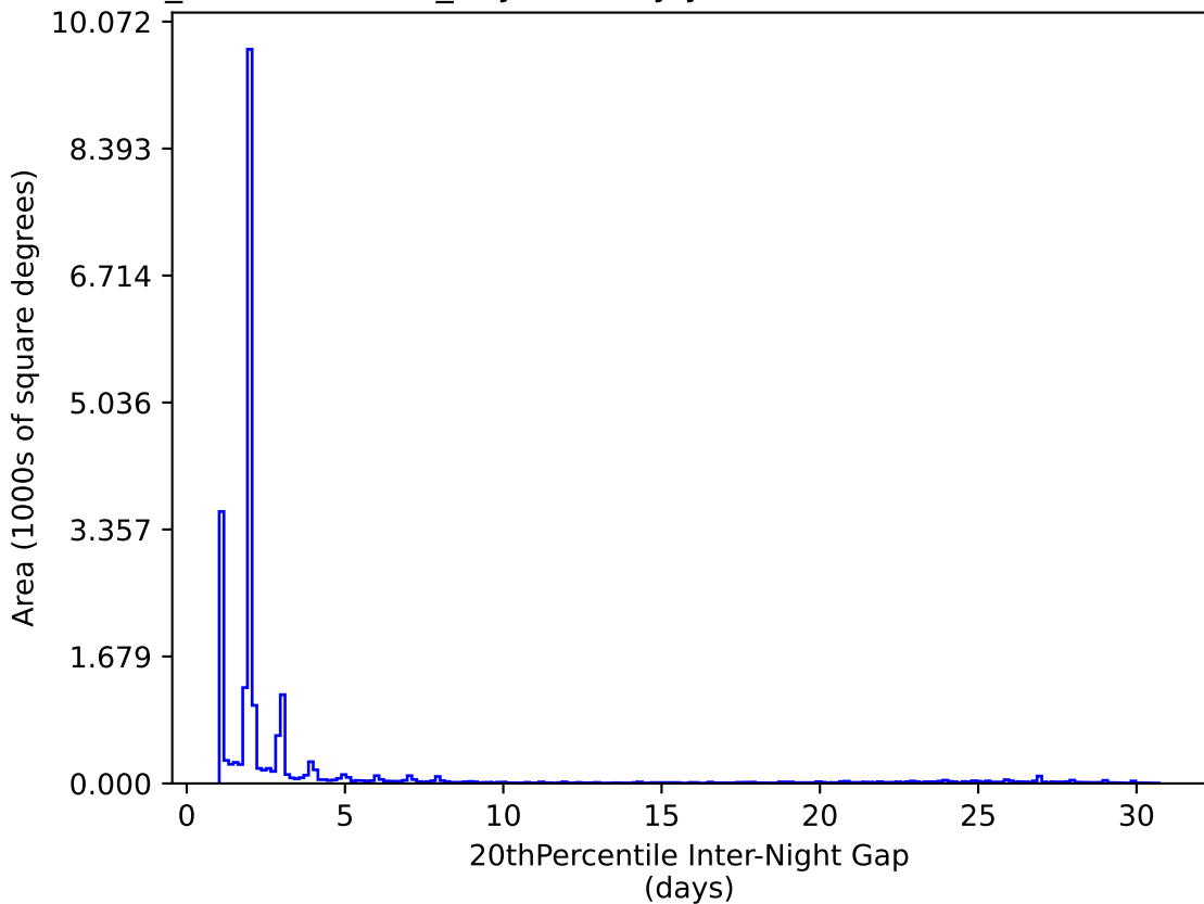
weather_cloudso10v3.4_10yrs All sky y band: 20thPercentile Inter-Night Gap
