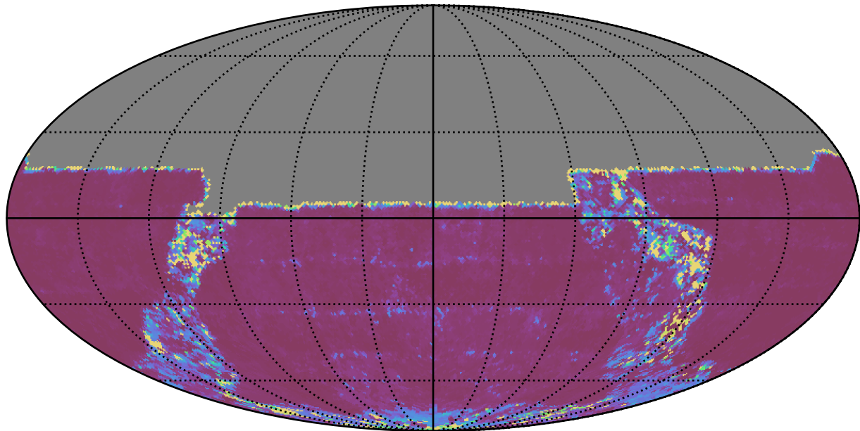
weather_cloudso10v3.4_10yrs All sky u band: 20thPercentile Inter-Night Gap
