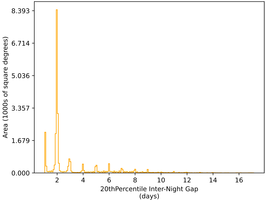
weather_cloudso10v3.4_10yrs All sky r band: 20thPercentile Inter-Night Gap
