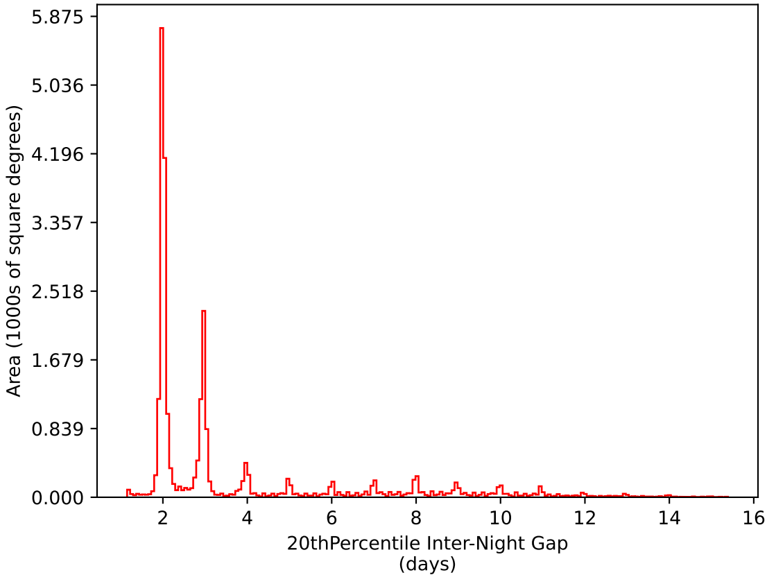
weather_cloudso10v3.4_10yrs All sky i band: 20thPercentile Inter-Night Gap
