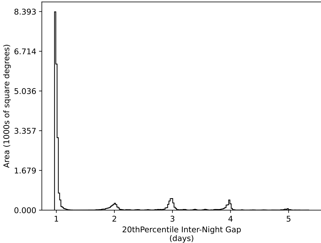
weather_cloudso10v3.4_10yrs All sky all bands: 20thPercentile Inter-Night Gap
