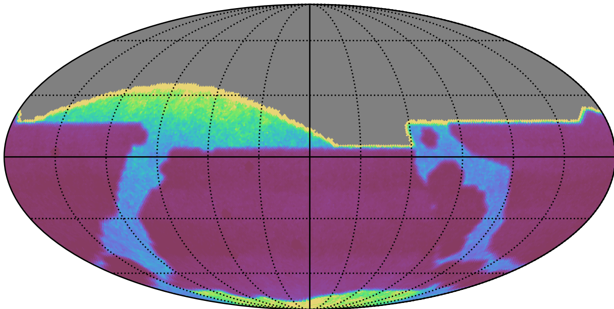
weather_cloudso10v3.4_10yrs : properMotion
