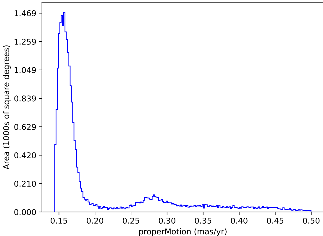
weather_cloudso10v3.4_10yrs : properMotion
