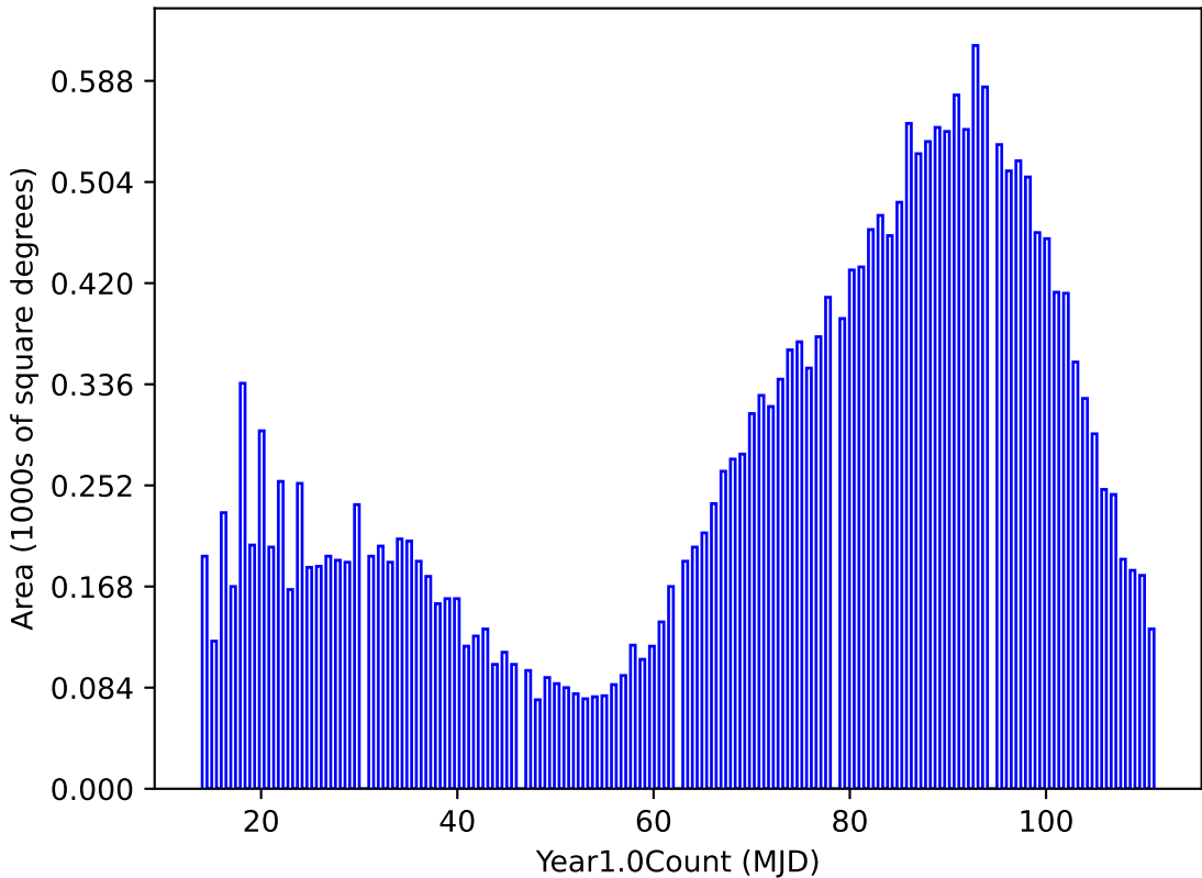
weather_cloudso10v3.4_10yrs night < 365.25: Year1.0Count
