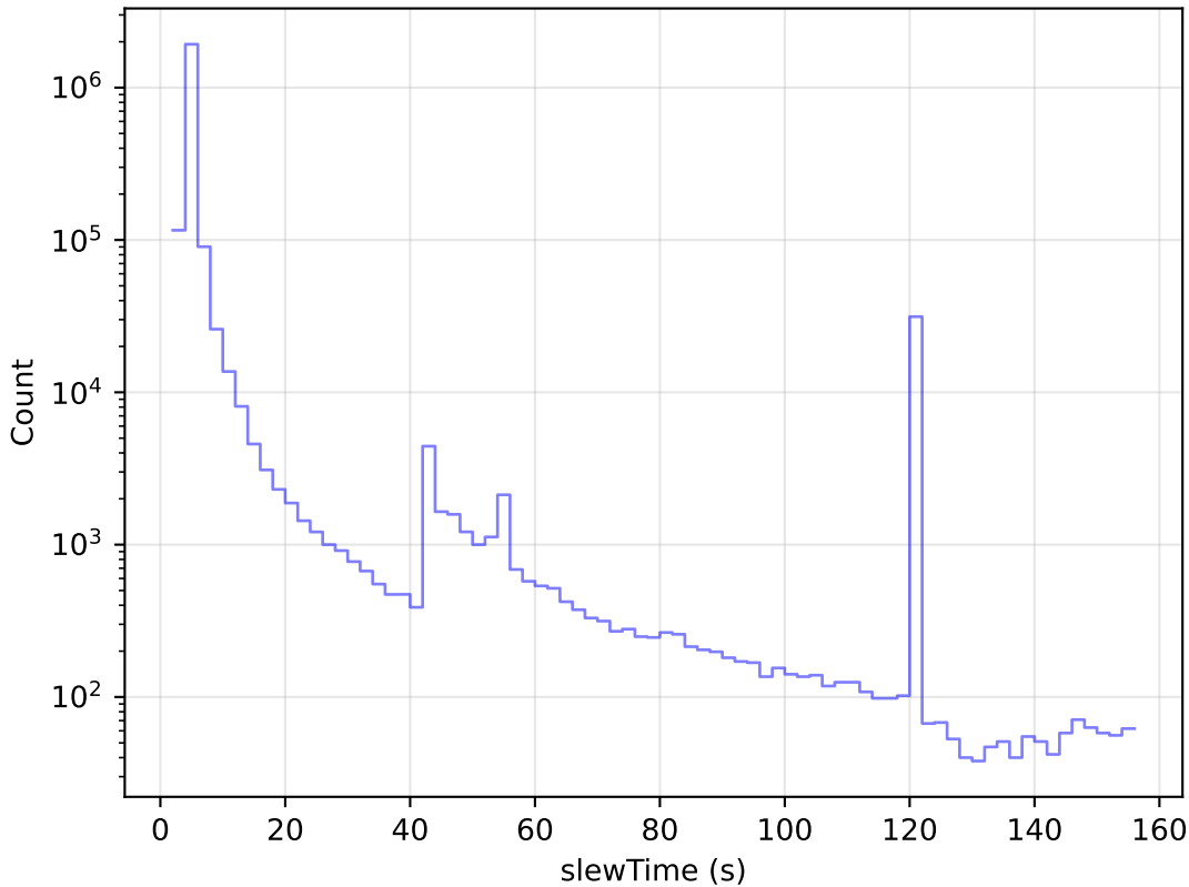
weather_cloudso10v3.4_10yrs All visits: Slew Time Histogram
