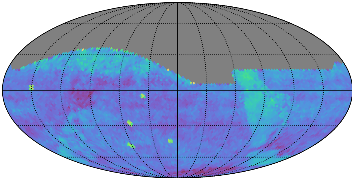
weather_cloudso10v3.4_10yrs (g or r or i): PairFraction
