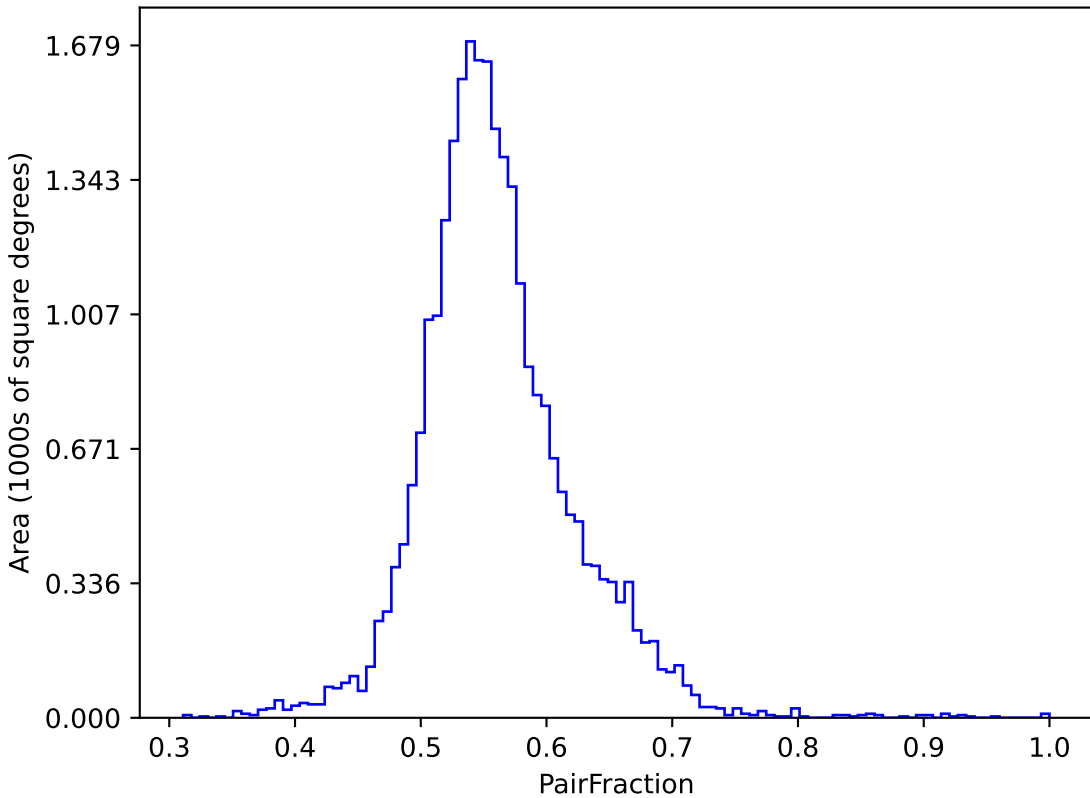
weather_cloudso10v3.4_10yrs (g or r or i): PairFraction
