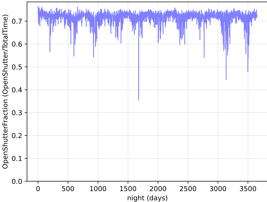
weather_cloudso10v3.4_10yrs : OpenShutterFraction
