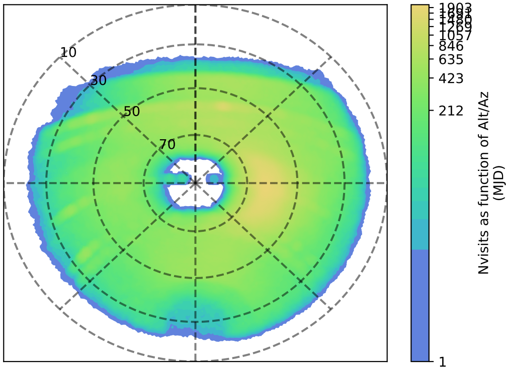
weather_cloudso10v3.4_10yrs y: Nvisits as function of Alt/Az
