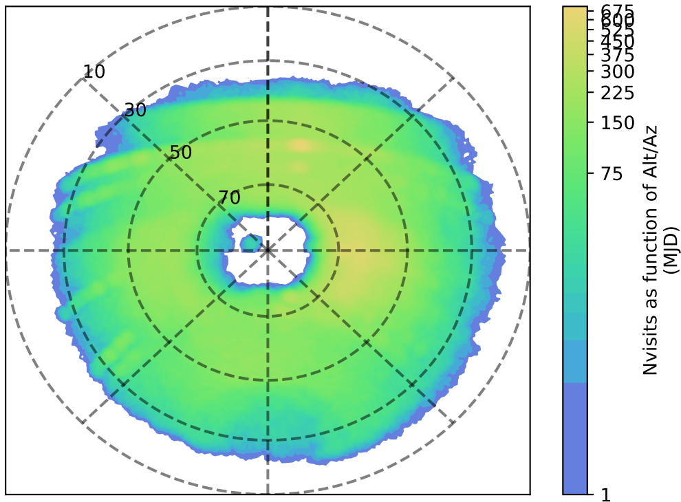
weather_cloudso10v3.4_10yrs u: Nvisits as function of Alt/Az
