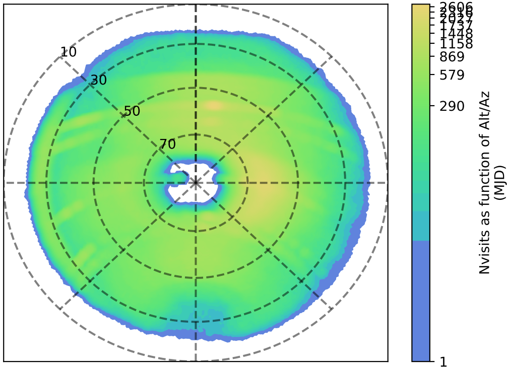
weather_cloudso10v3.4_10yrs r: Nvisits as function of Alt/Az
