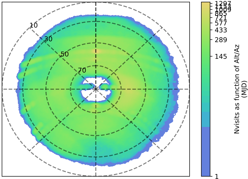
weather_cloudso10v3.4_10yrs g: Nvisits as function of Alt/Az
