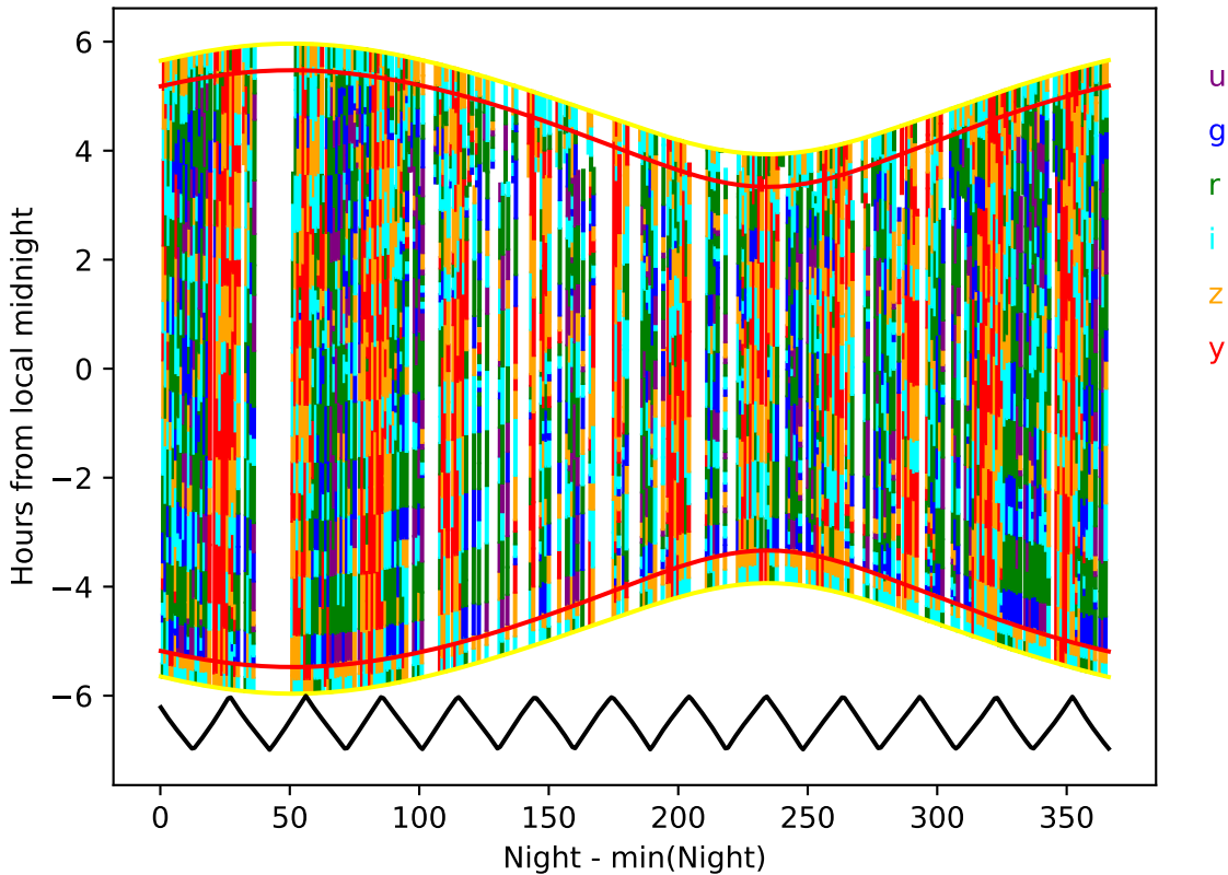
weather_cloudso10v3.4_10yrs year 4-5: Hourglass
