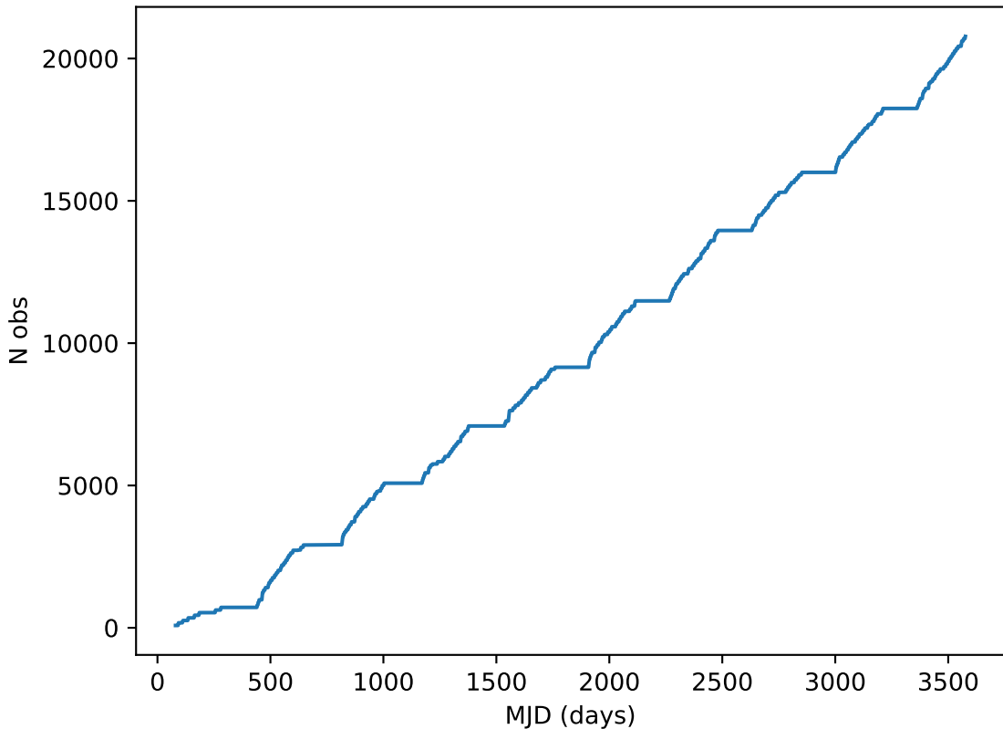
weather_cloudso10v3.4_10yrs note like DD:XMM_LSS%: Cumulative
