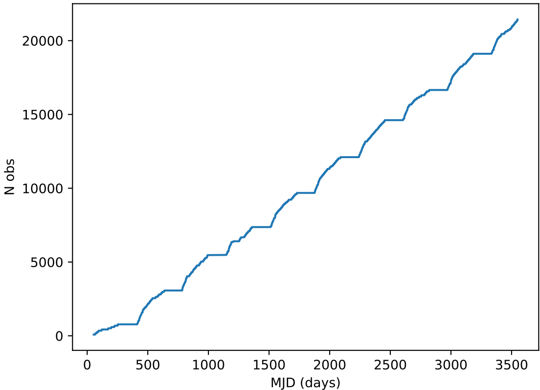
weather_cloudso10v3.4_10yrs note like DD:ELAISS1%: Cumulative
