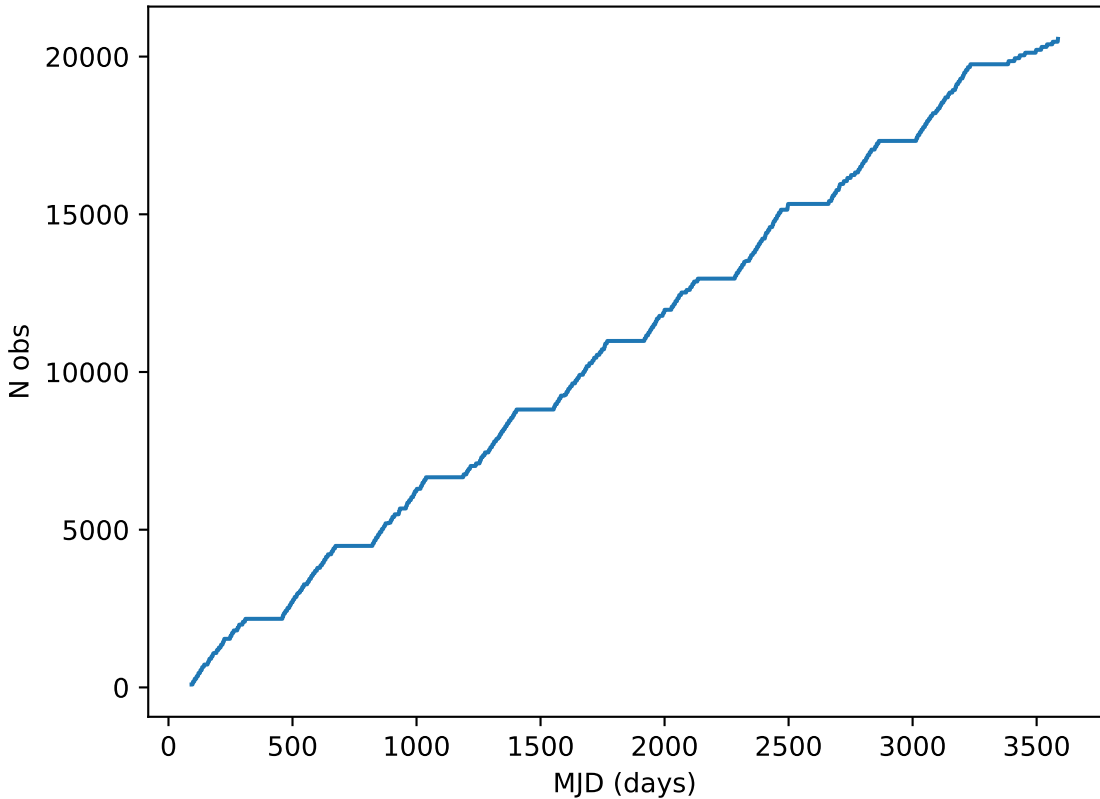
weather_cloudso10v3.4_10yrs note like DD:ECDFS%: Cumulative
