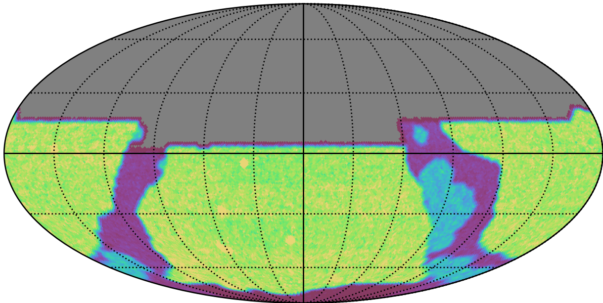
weather_cloudso10v3.4_10yrs y: Count observationStartMJD
