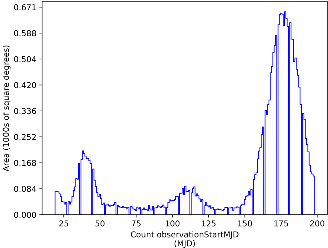
weather_cloudso10v3.4_10yrs y: Count observationStartMJD
