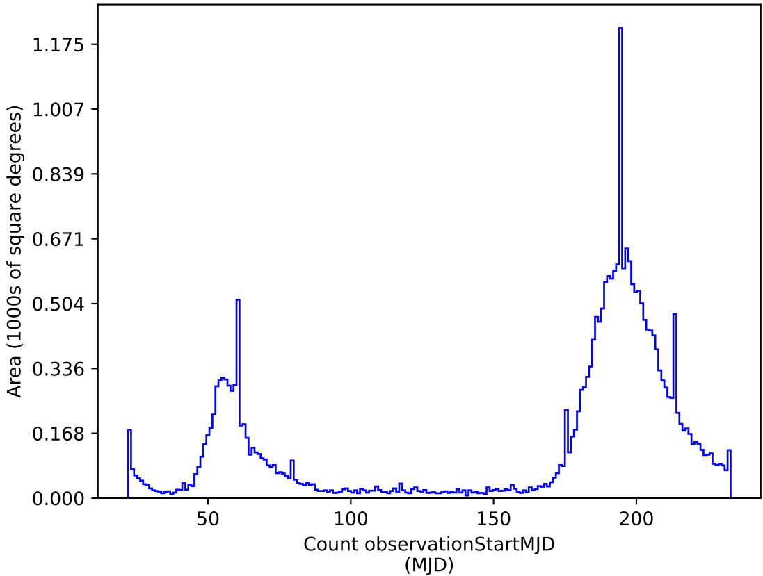
weather_cloudso10v3.4_10yrs r: Count observationStartMJD
