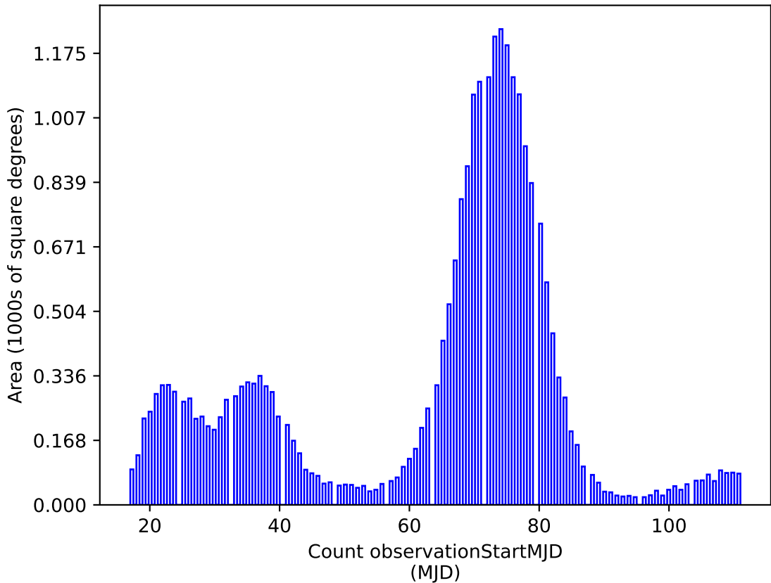
weather_cloudso10v3.4_10yrs g: Count observationStartMJD
