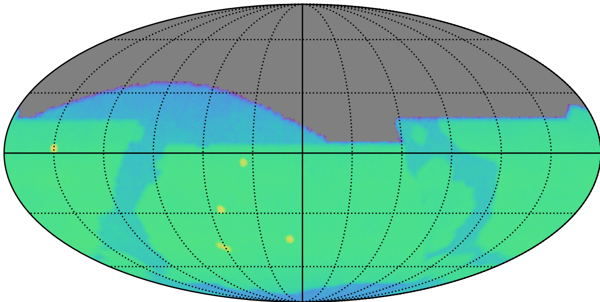
weather_cloudso10v3.4_10yrs z: CoaddM5
