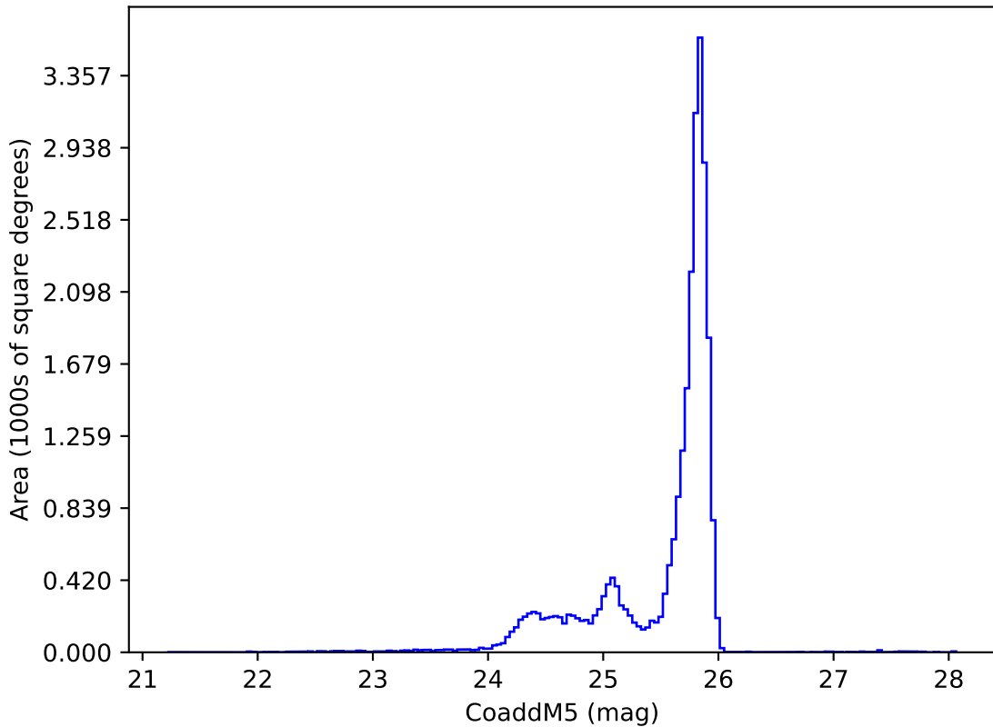
weather_cloudso10v3.4_10yrs z: CoaddM5
