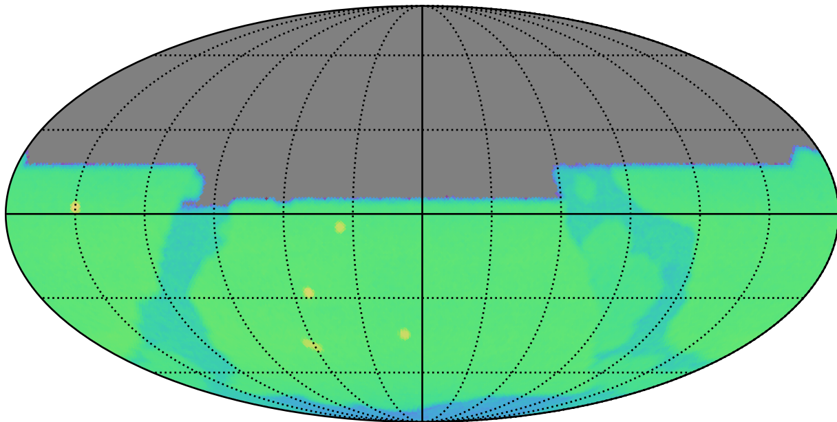
weather_cloudso10v3.4_10yrs y: CoaddM5
