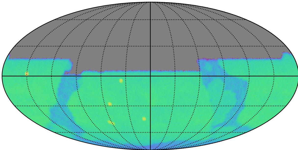
weather_cloudso10v3.4_10yrs u: CoaddM5
