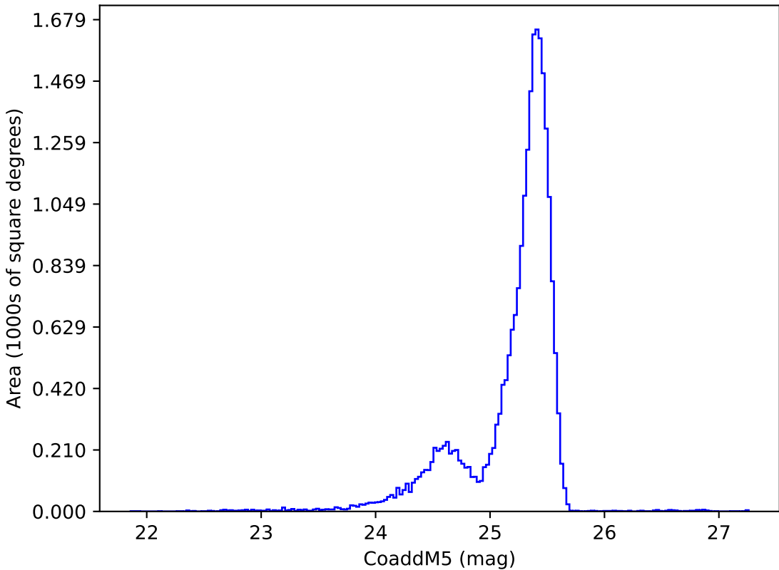
weather_cloudso10v3.4_10yrs u: CoaddM5
