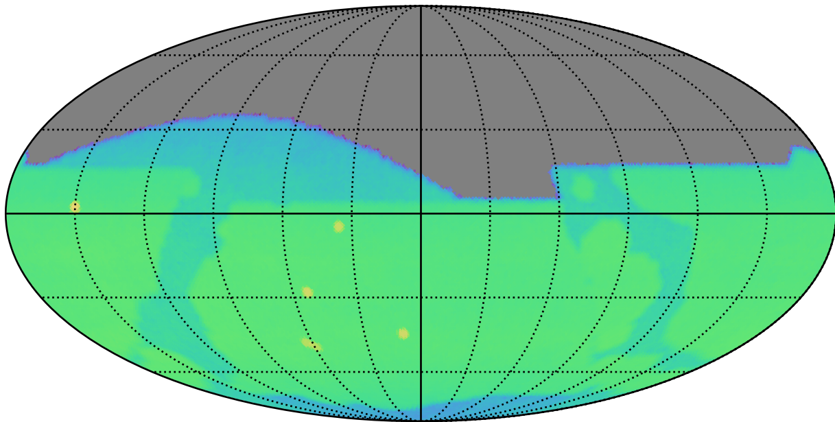
weather_cloudso10v3.4_10yrs r: CoaddM5
