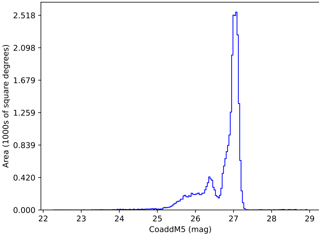
weather_cloudso10v3.4_10yrs r: CoaddM5
