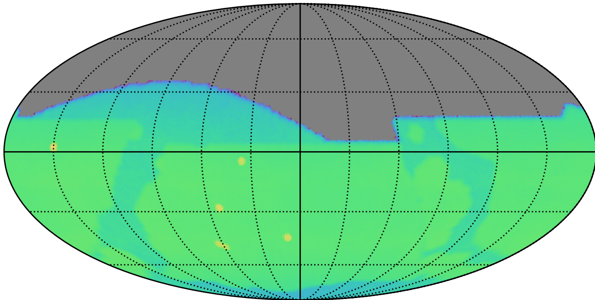
weather_cloudso10v3.4_10yrs : CoaddM5
