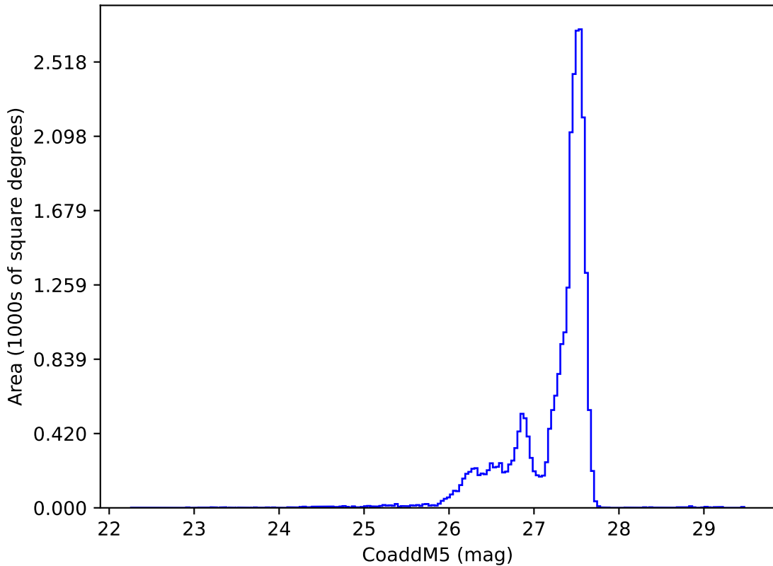
weather_cloudso10v3.4_10yrs : CoaddM5
